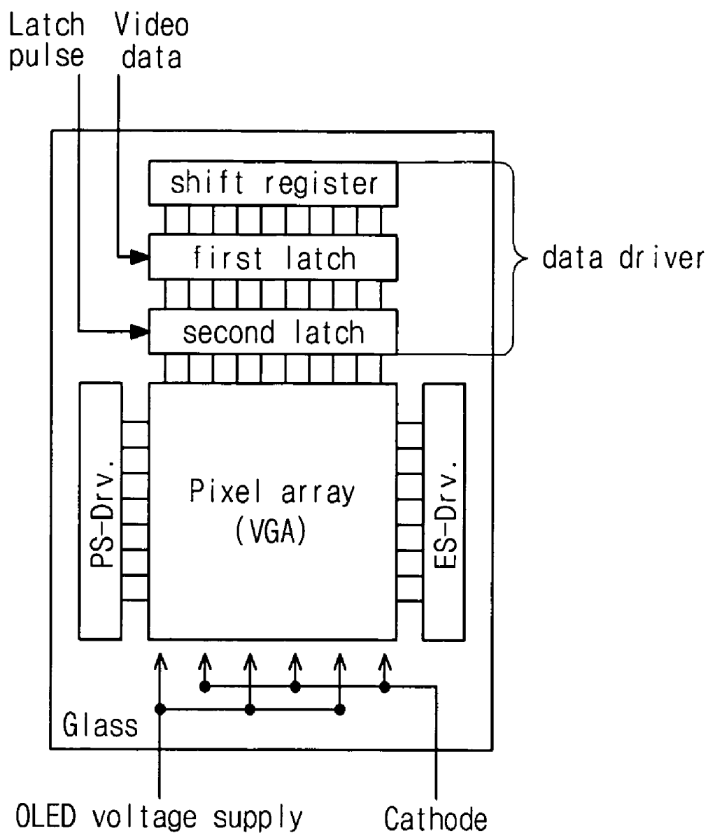
FIG. 8 (RELATED ART)
