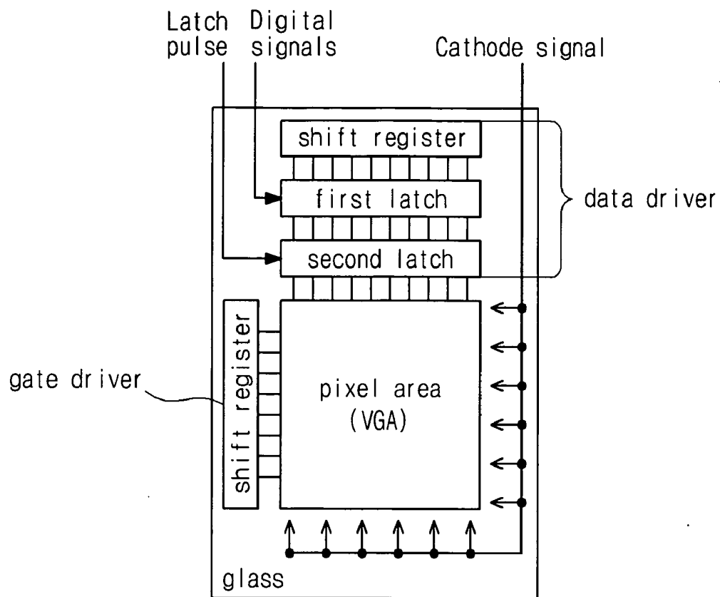
FIG. 5 (RELATED ART)
