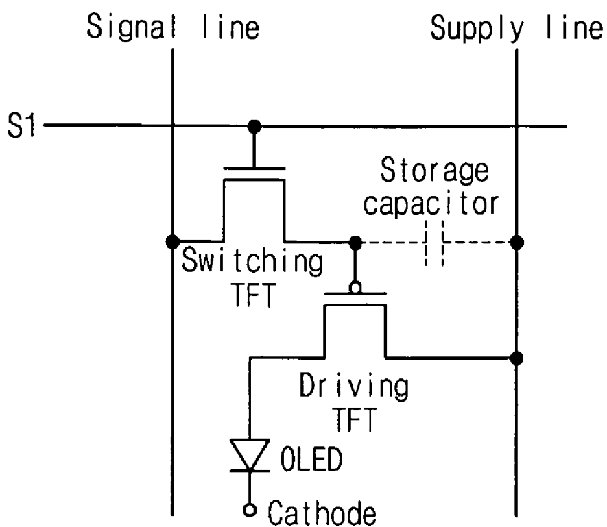
FIG. 3 (RELATED ART)
