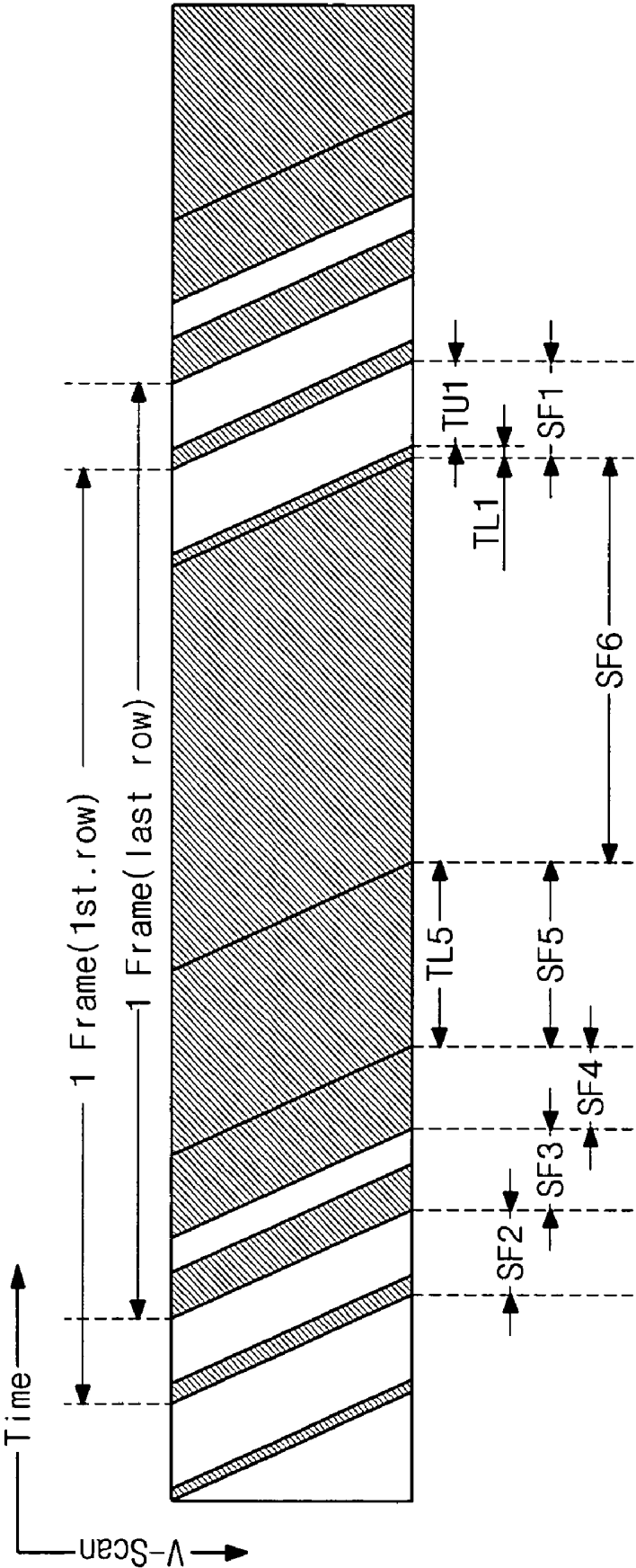
FIG. 7 (RELATED ART)
