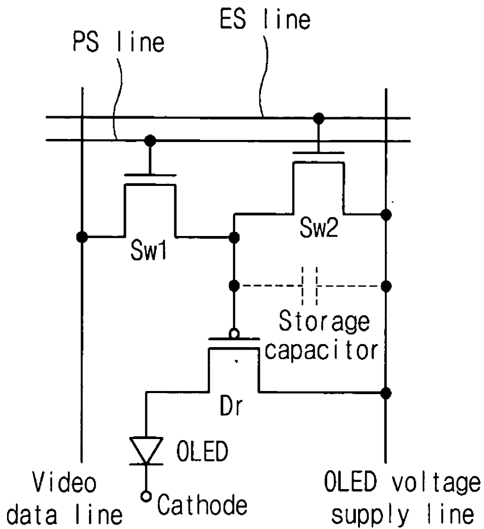
FIG. 6 (RELATED ART)
