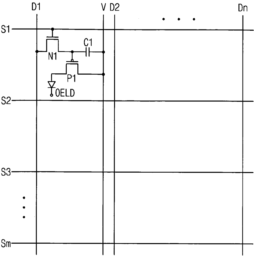
FIG. 1 (RELATED ART)
