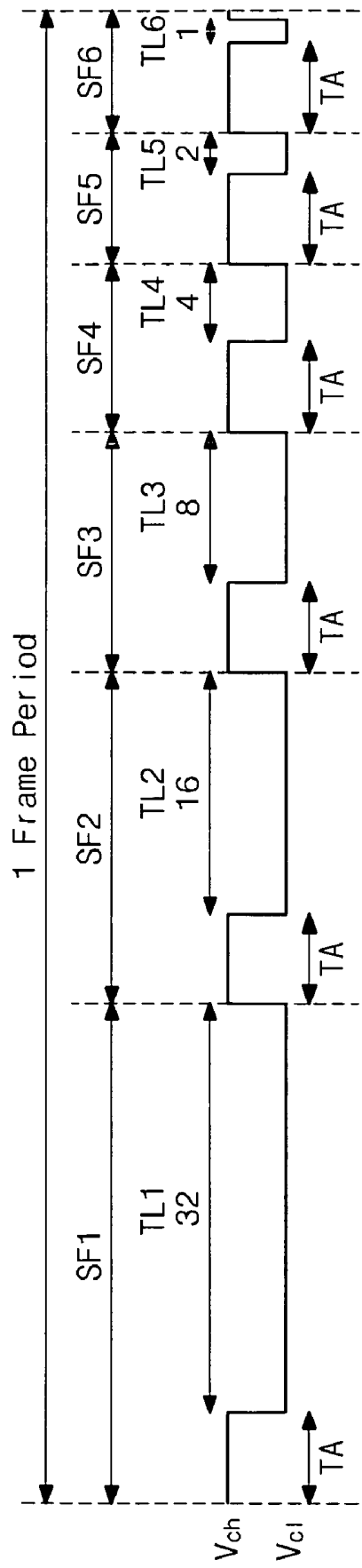
FIG. 4 (RELATED ART)
